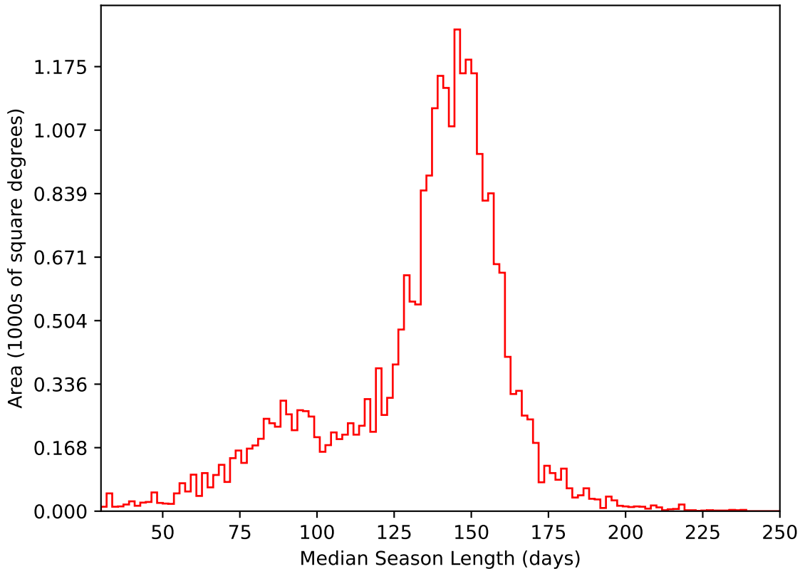
ddf_acor_sf25_lsf40_lsr10_v3.4_10yrs All sky i band: Median Season Length
