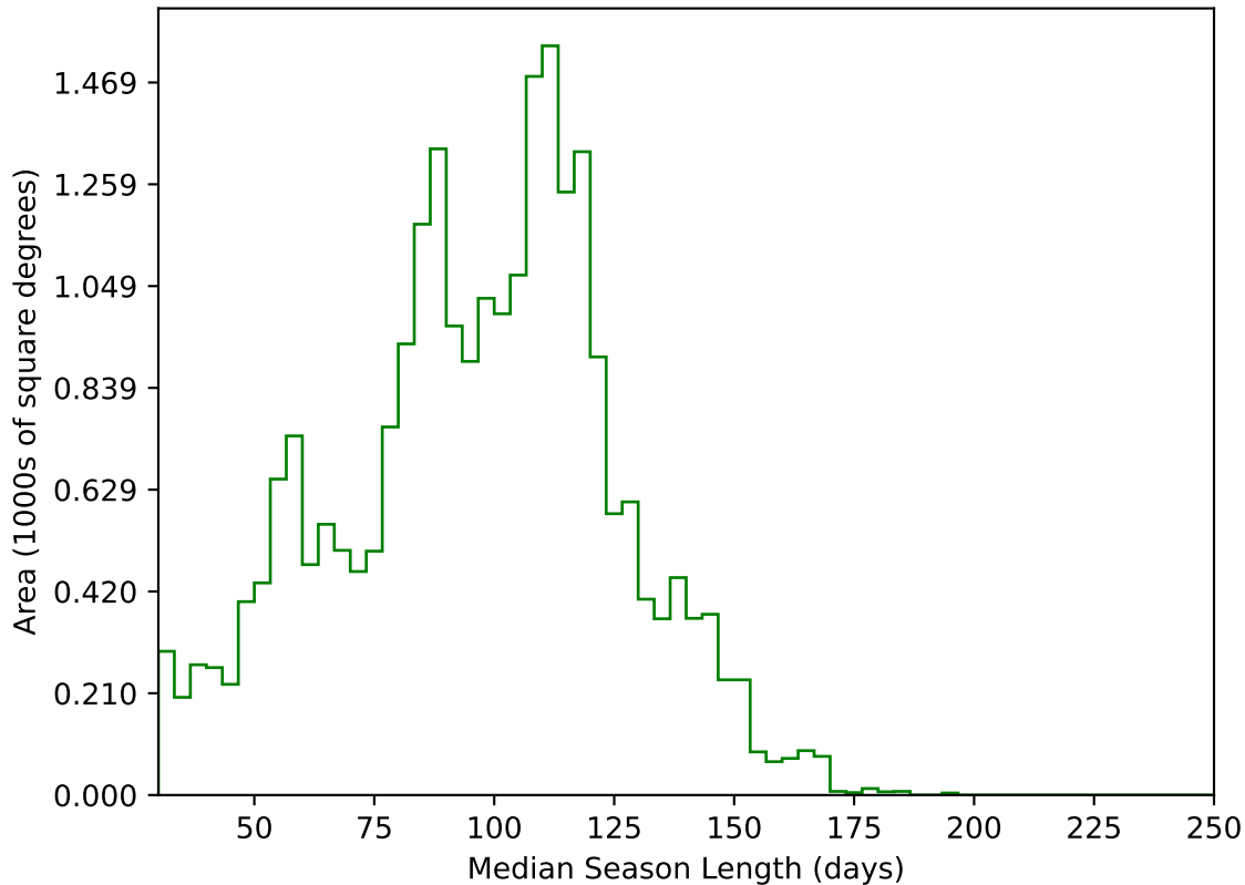
ddf_acor_sf25_lsf40_lsr10_v3.4_10yrs All sky g band: Median Season Length
