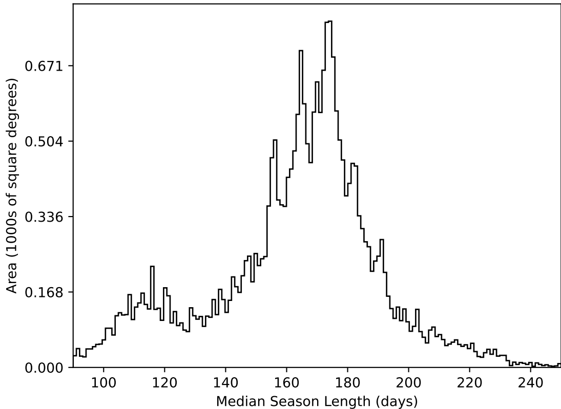
ddf_acor_sf25_lsf40_lsr10_v3.4_10yrs All sky all bands: Median Season Length
