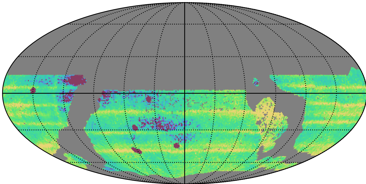
ddf_acor_sf25_lsf40_lsr10_v3.4_10yrs WFD: Median Intra-Night Gap
