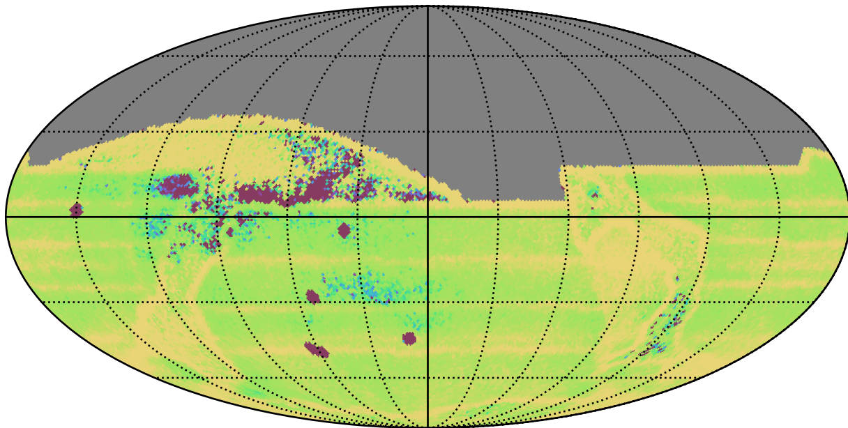
ddf_acor_sf25_lsf40_lsr10_v3.4_10yrs All sky: Median Intra-Night Gap
