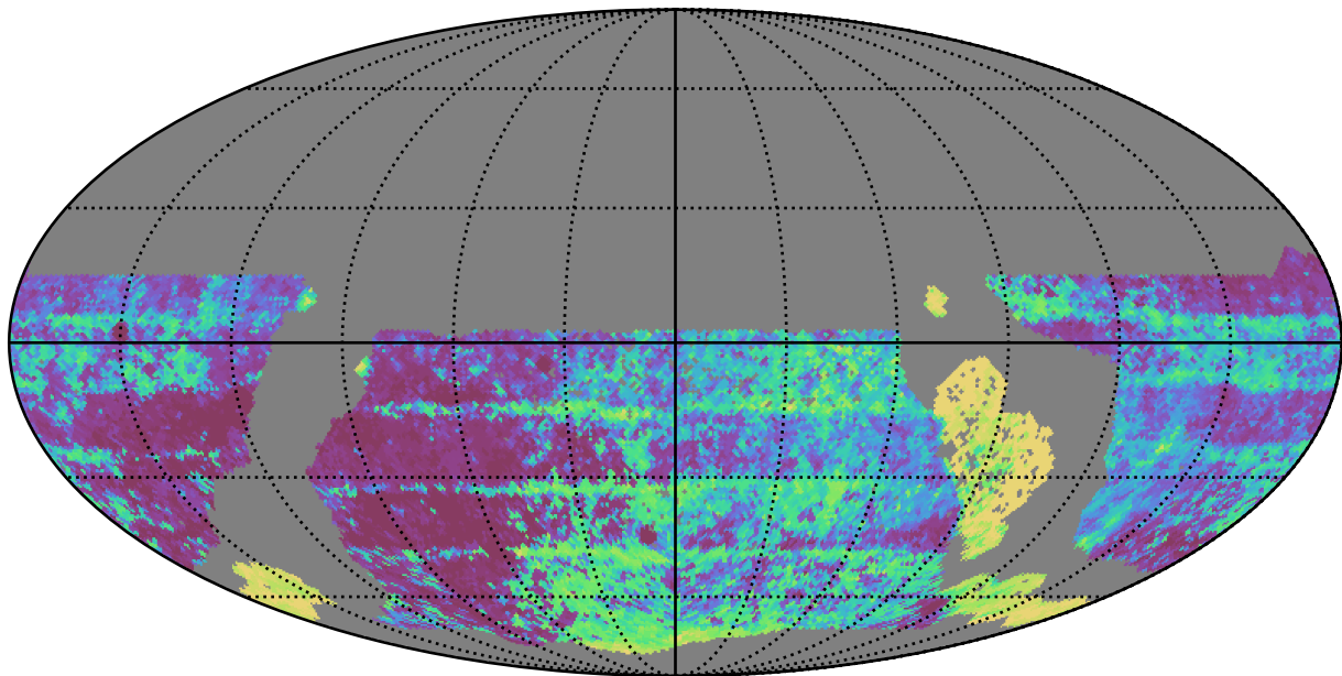
ddf_acor_sf25_lsf40_lsr10_v3.4_10yrs WFD y band: Median Inter-Night Gap
