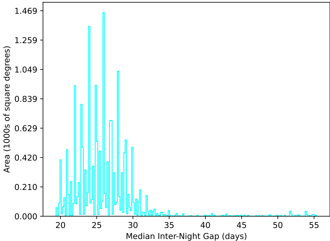
ddf_acor_sf25_lsf40_lsr10_v3.4_10yrs WFD u band: Median Inter-Night Gap
