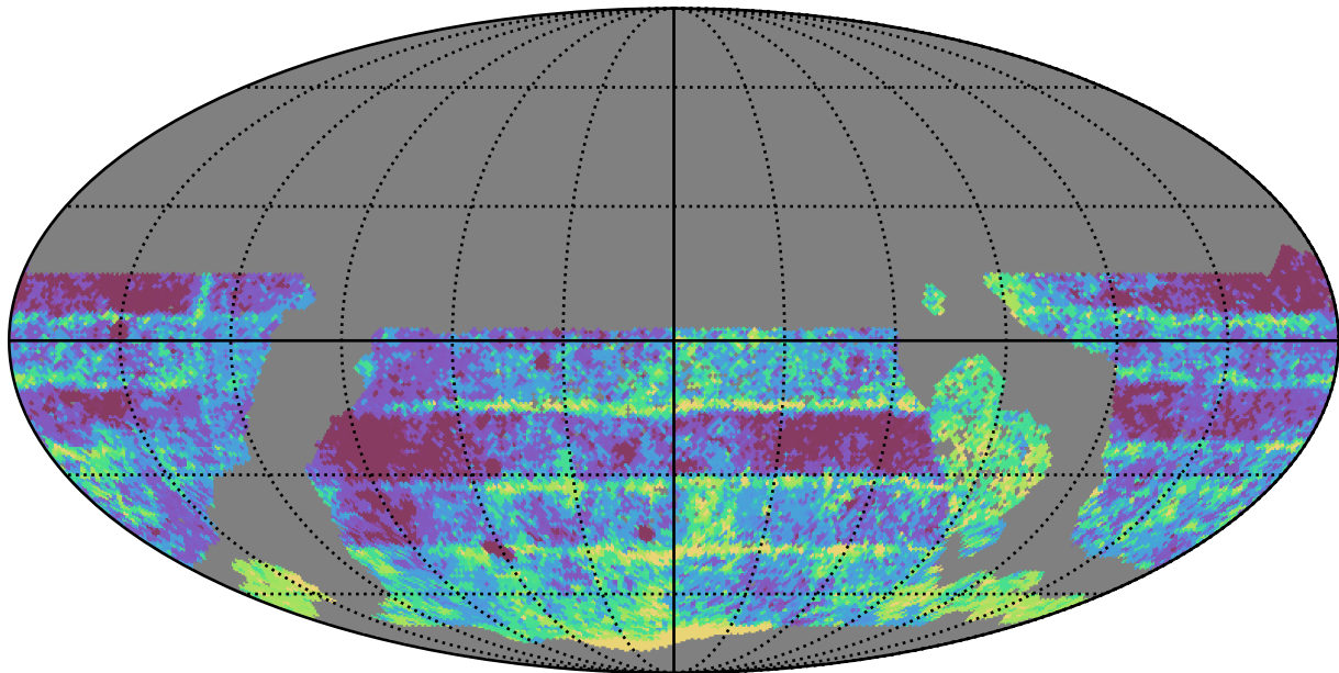
ddf_acor_sf25_lsf40_lsr10_v3.4_10yrs WFD r band: Median Inter-Night Gap
