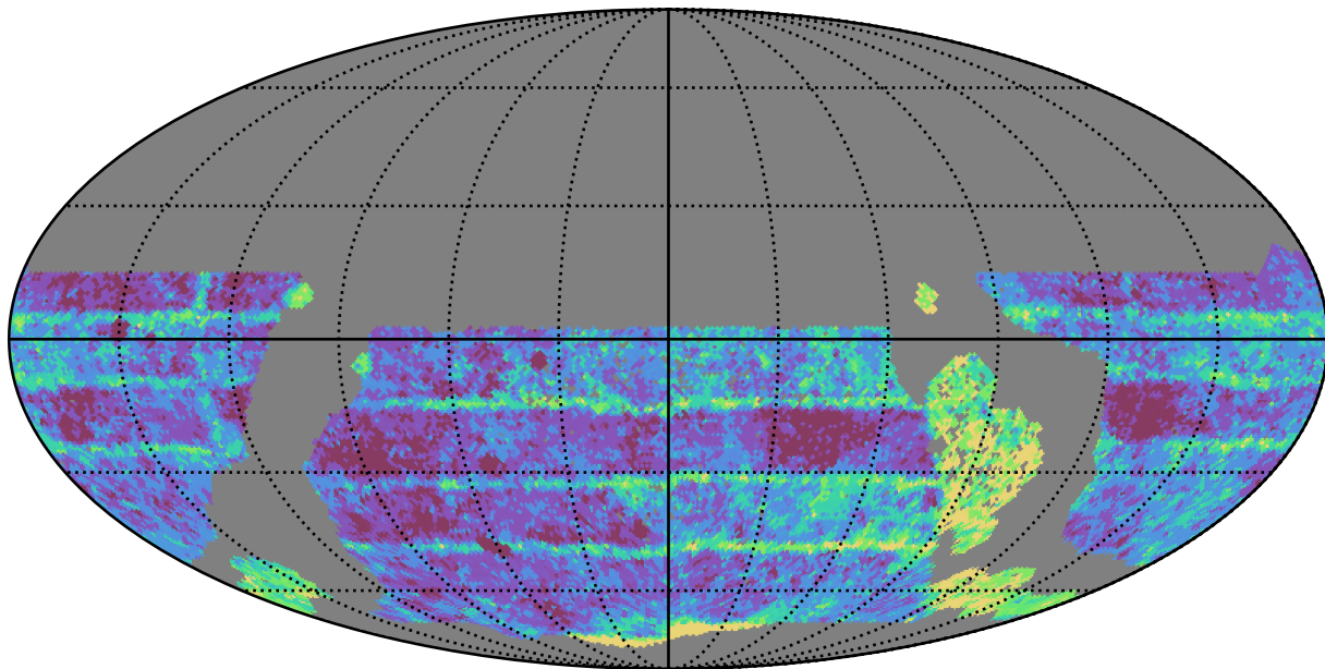
ddf_acor_sf25_lsf40_lsr10_v3.4_10yrs WFD i band: Median Inter-Night Gap
