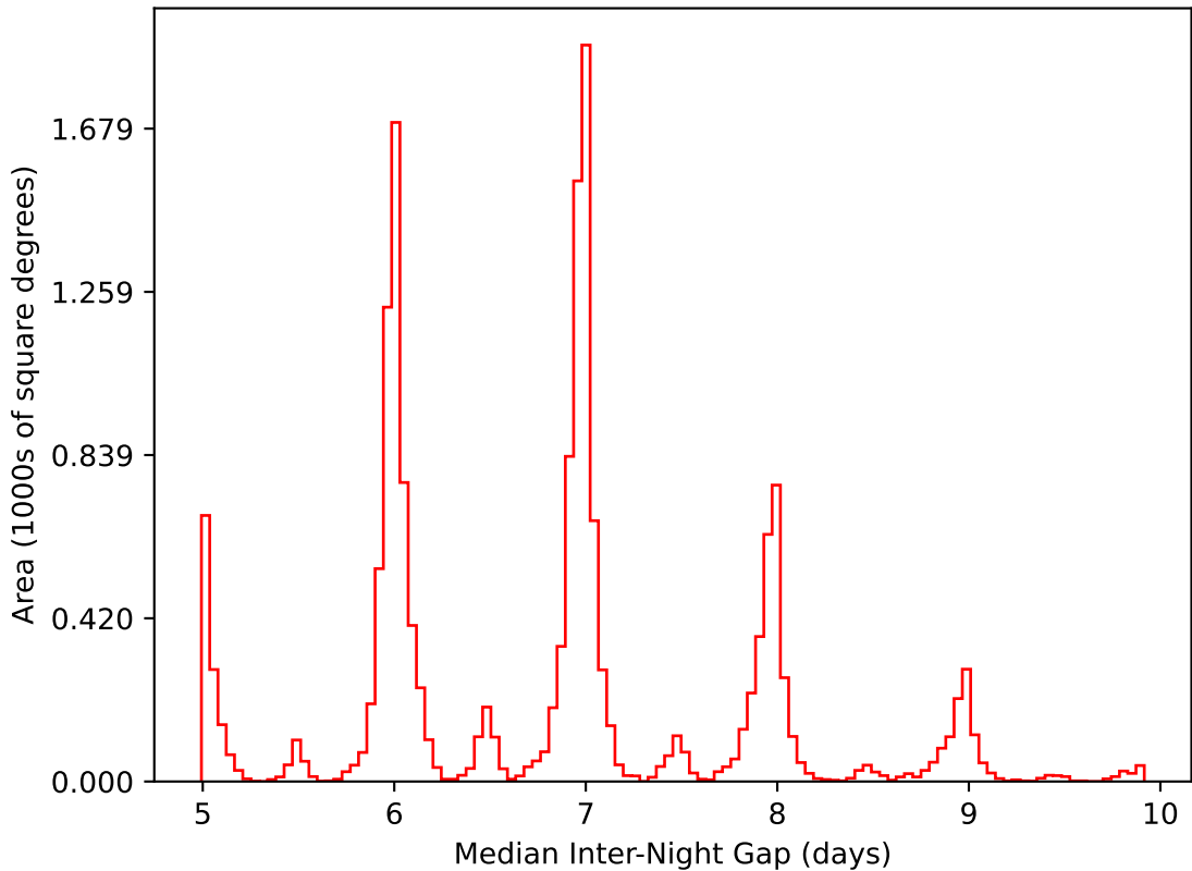
ddf_acor_sf25_lsf40_lsr10_v3.4_10yrs WFD i band: Median Inter-Night Gap
