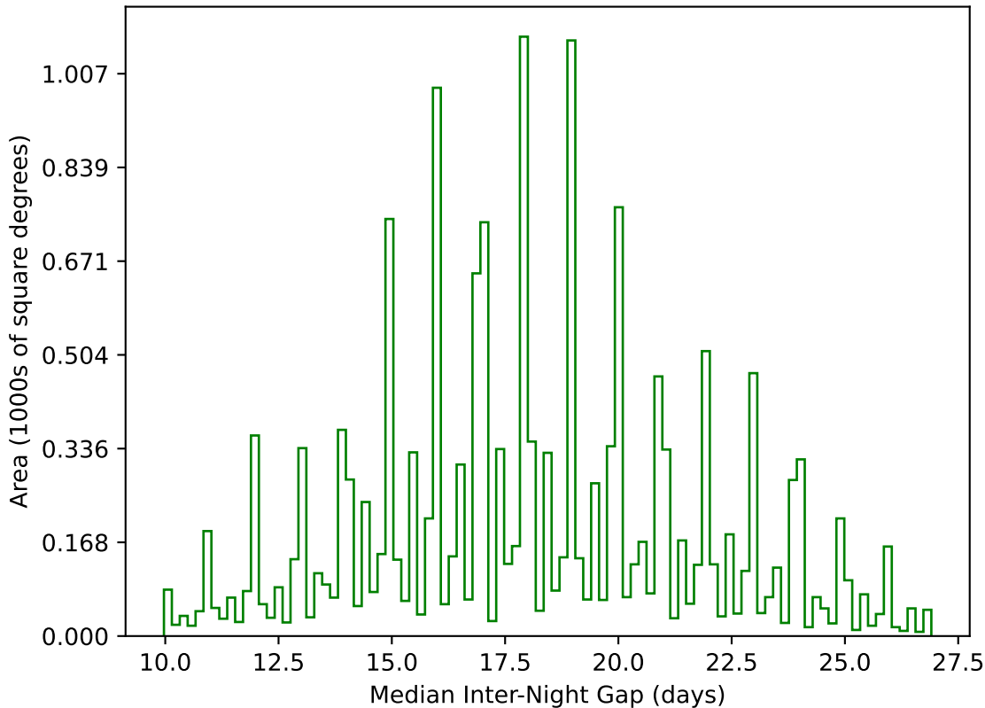
ddf_acor_sf25_lsf40_lsr10_v3.4_10yrs WFD g band: Median Inter-Night Gap
