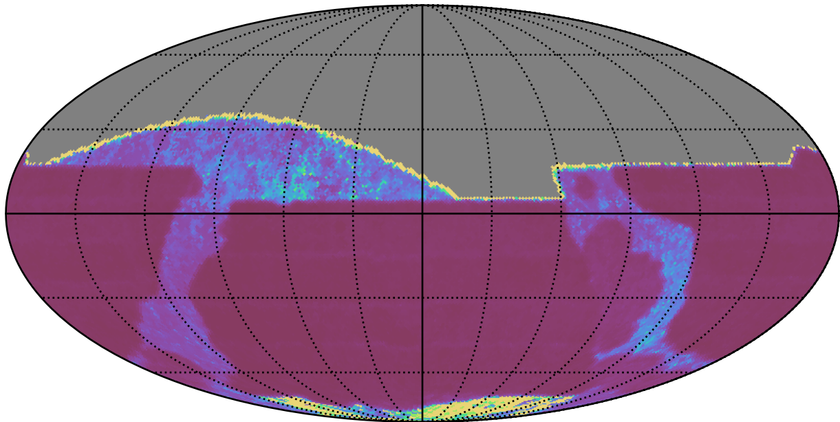
ddf_acor_sf25_lsf40_lsr10_v3.4_10yrs All sky z band: Median Inter-Night Gap
