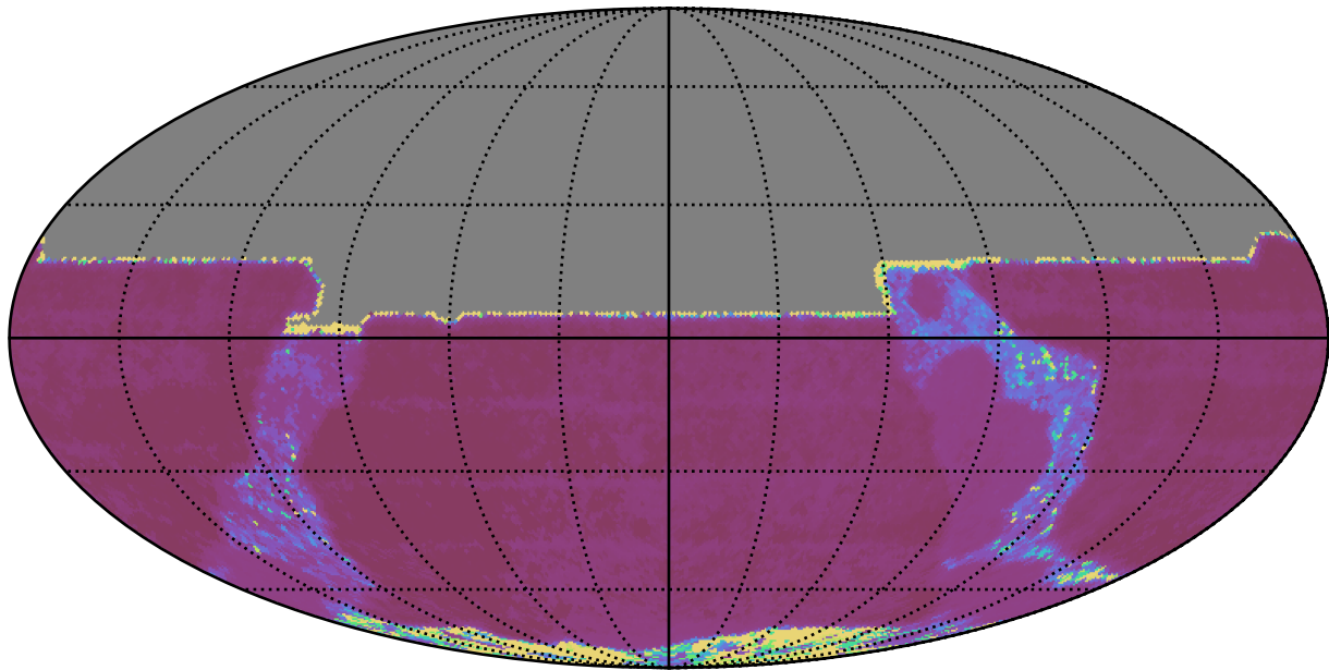
ddf_acor_sf25_lsf40_lsr10_v3.4_10yrs All sky y band: Median Inter-Night Gap
