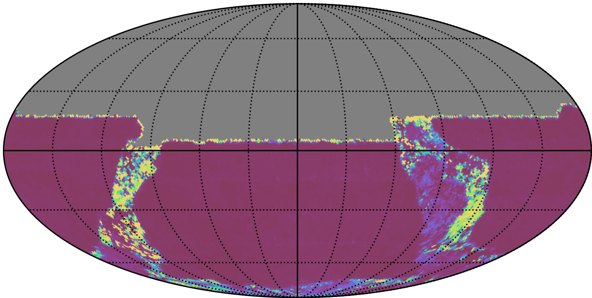
ddf_acor_sf25_lsf40_lsr10_v3.4_10yrs All sky u band: Median Inter-Night Gap
