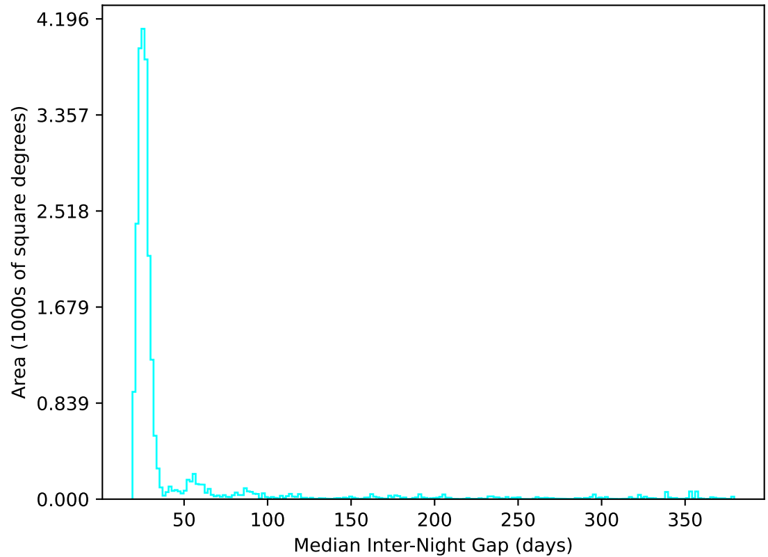
ddf_acor_sf25_lsf40_lsr10_v3.4_10yrs All sky u band: Median Inter-Night Gap
