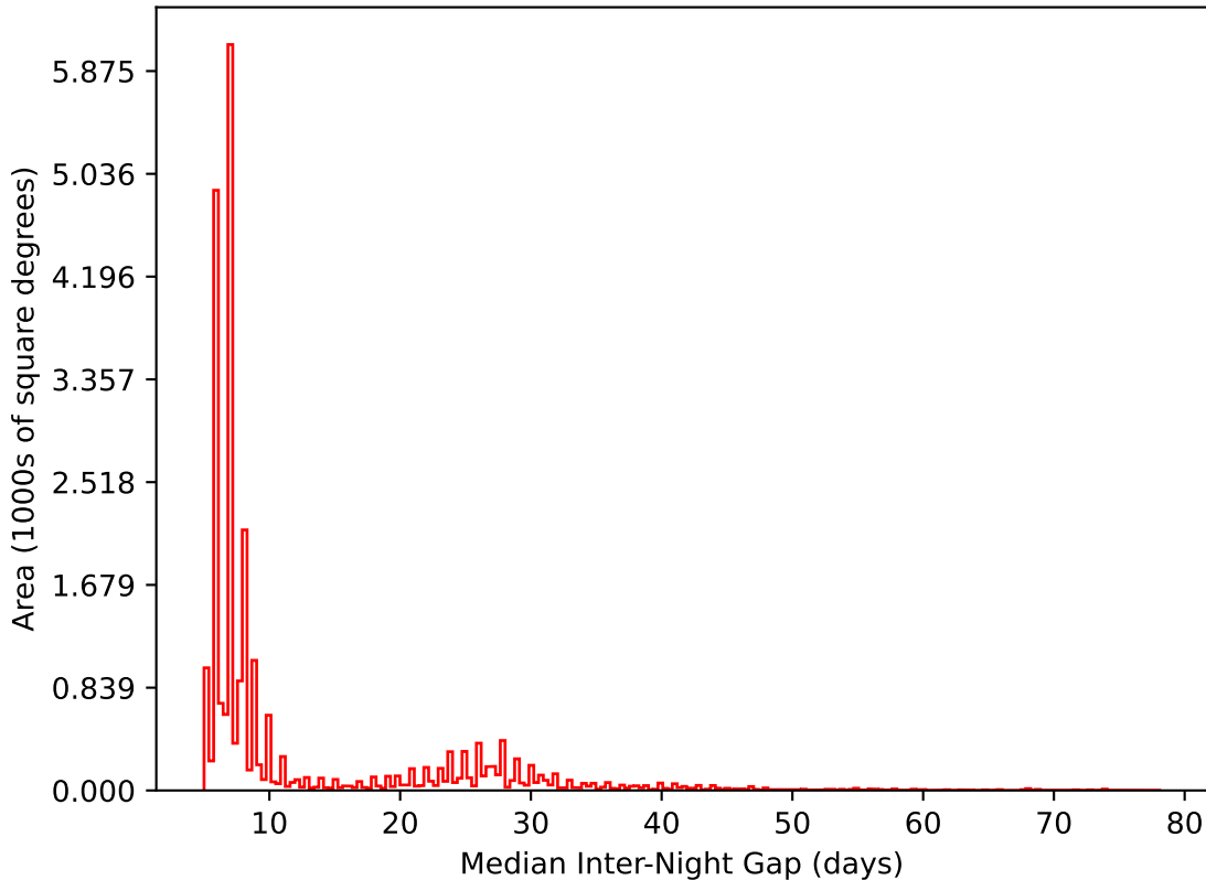
ddf_acor_sf25_lsf40_lsr10_v3.4_10yrs All sky i band: Median Inter-Night Gap
