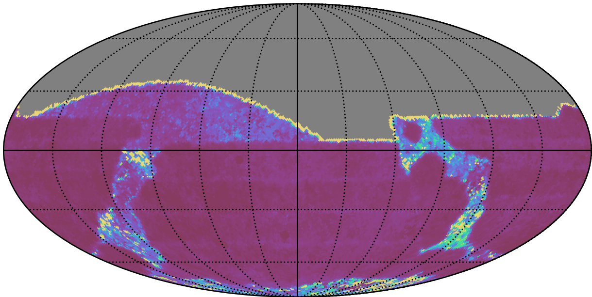
ddf_acor_sf25_lsf40_lsr10_v3.4_10yrs All sky g band: Median Inter-Night Gap
