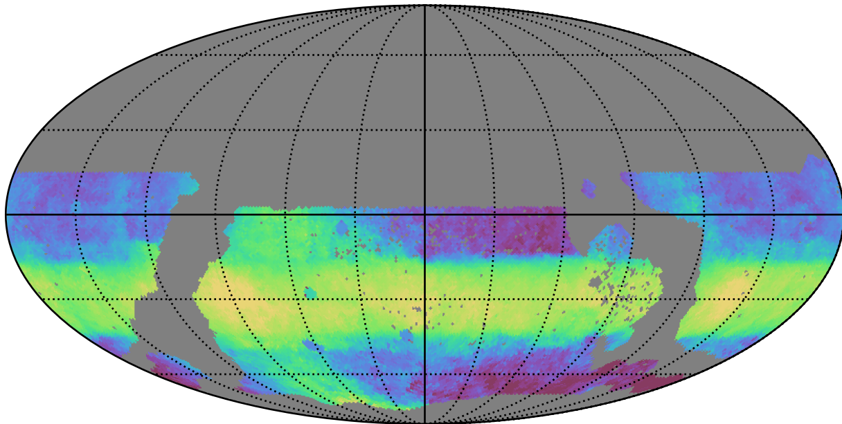
ddf_acor_sf25_lsf40_lsr10_v3.4_10yrs WFD z band: Median HA
