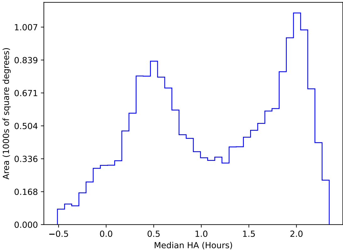
ddf_acor_sf25_lsf40_lsr10_v3.4_10yrs WFD z band: Median HA
