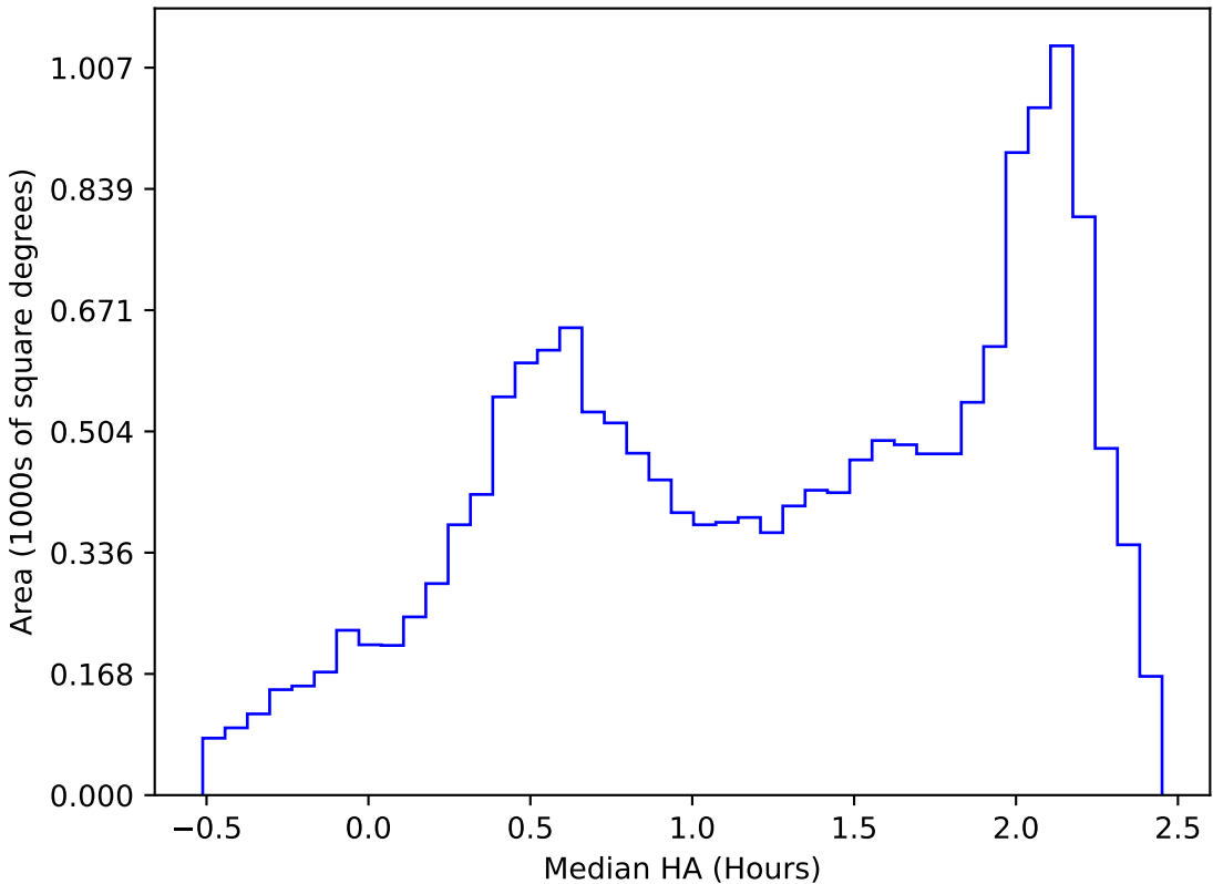
ddf_acor_sf25_lsf40_lsr10_v3.4_10yrs WFD y band: Median HA
