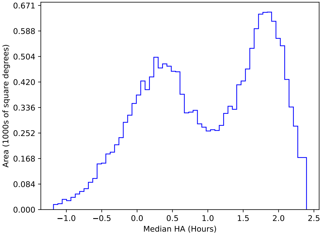
ddf_acor_sf25_lsf40_lsr10_v3.4_10yrs WFD u band: Median HA
