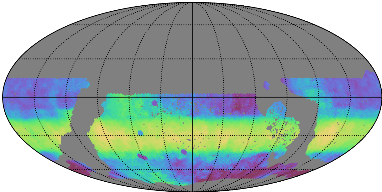
ddf_acor_sf25_lsf40_lsr10_v3.4_10yrs WFD i band: Median HA
