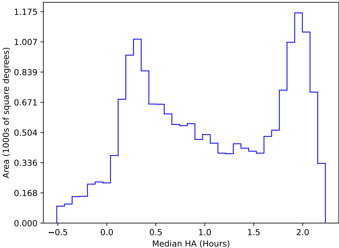
ddf_acor_sf25_lsf40_lsr10_v3.4_10yrs WFD i band: Median HA
