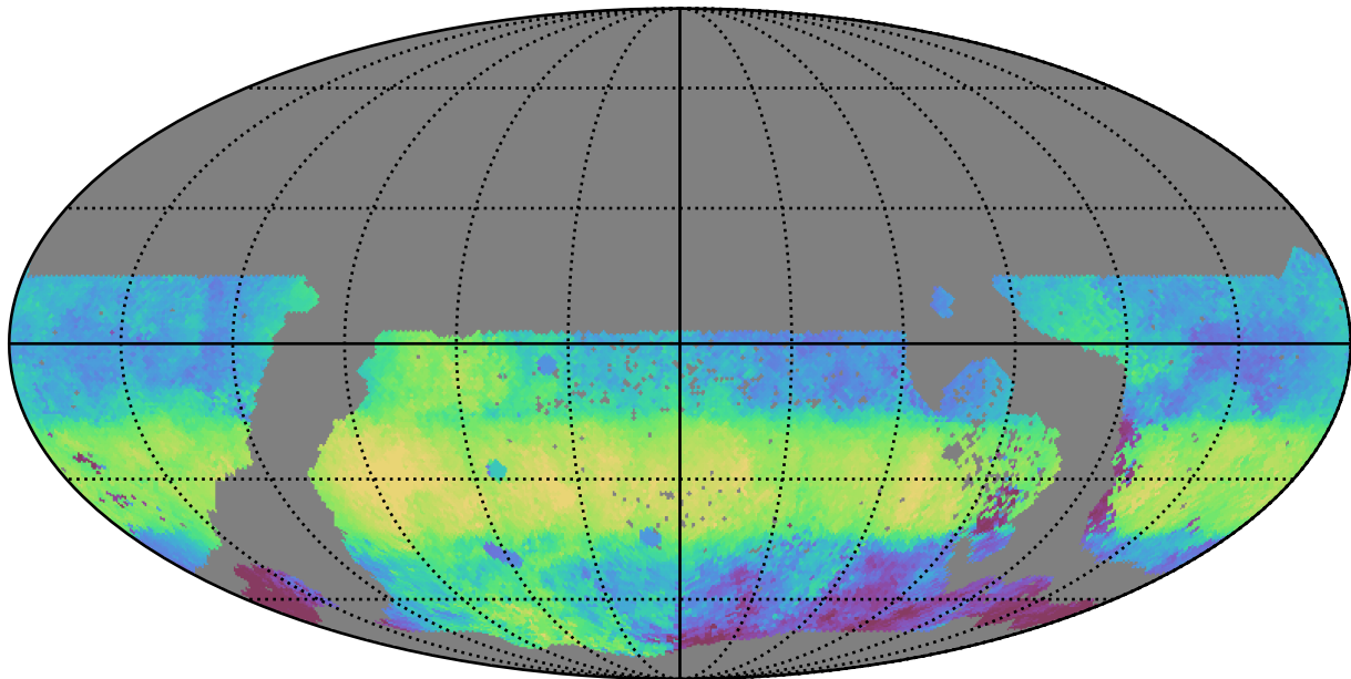
ddf_acor_sf25_lsf40_lsr10_v3.4_10yrs WFD g band: Median HA
