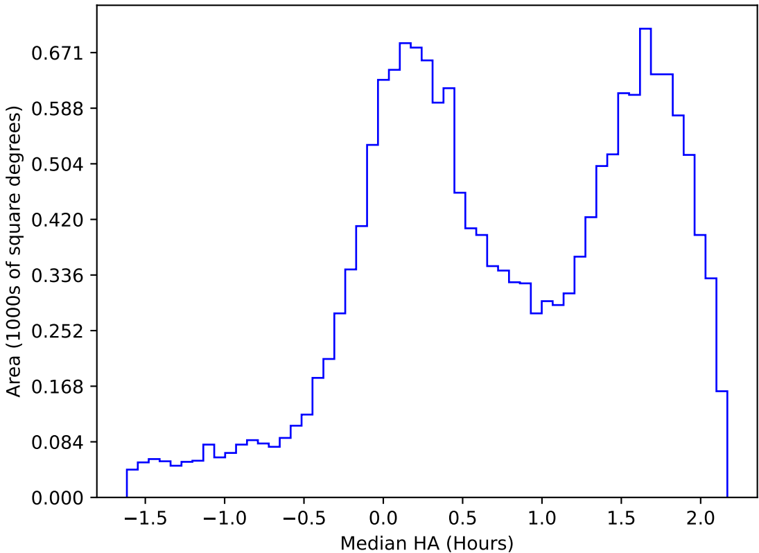
ddf_acor_sf25_lsf40_lsr10_v3.4_10yrs WFD g band: Median HA
