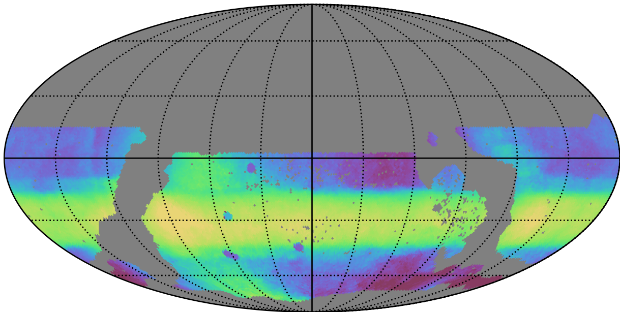
ddf_acor_sf25_lsf40_lsr10_v3.4_10yrs WFD all bands: Median HA
