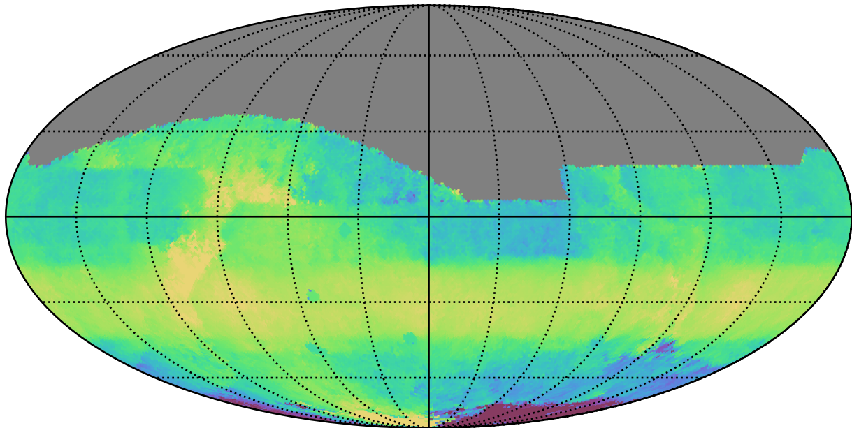
ddf_acor_sf25_lsf40_lsr10_v3.4_10yrs All sky z band: Median HA
