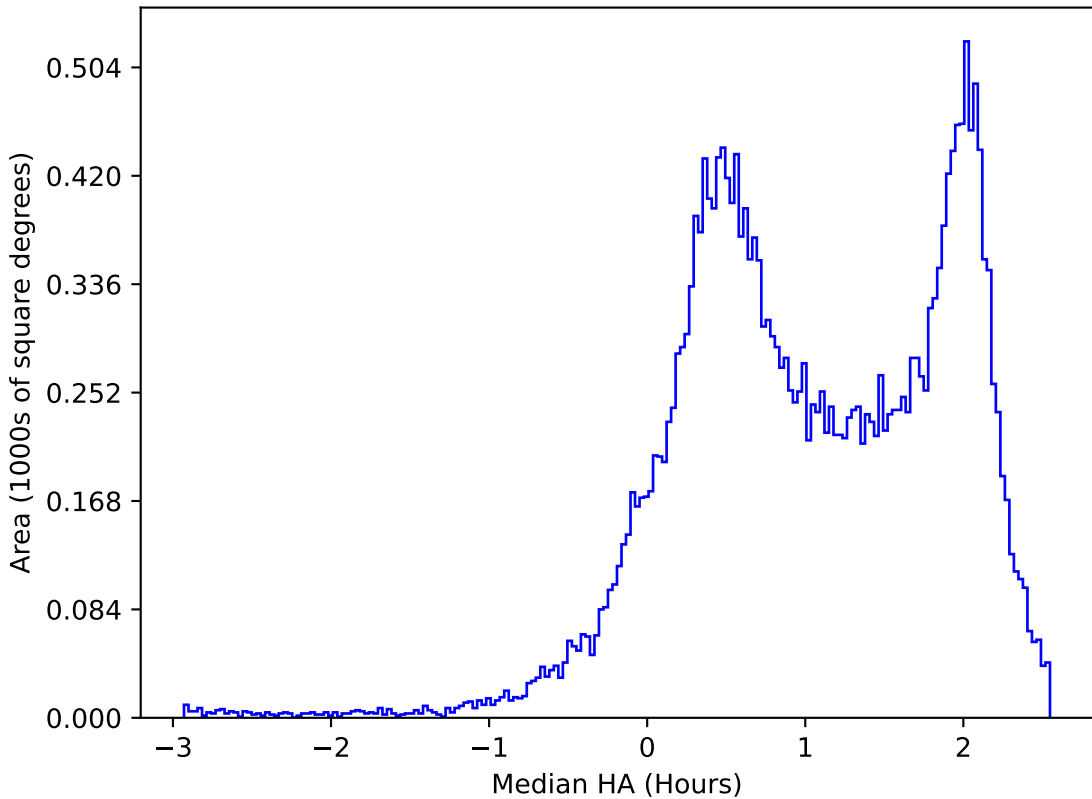
ddf_acor_sf25_lsf40_lsr10_v3.4_10yrs All sky z band: Median HA
