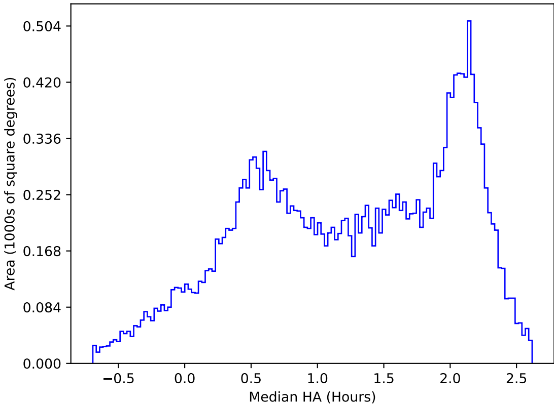
ddf_acor_sf25_lsf40_lsr10_v3.4_10yrs All sky y band: Median HA
