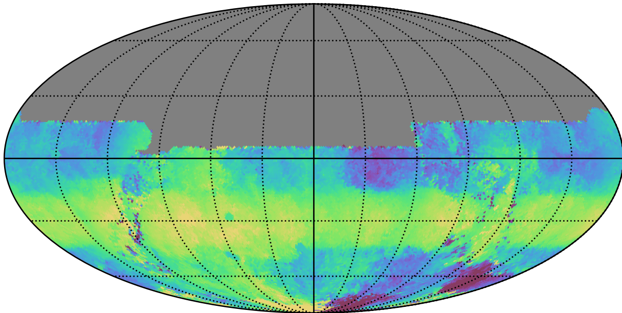
ddf_acor_sf25_lsf40_lsr10_v3.4_10yrs All sky u band: Median HA
