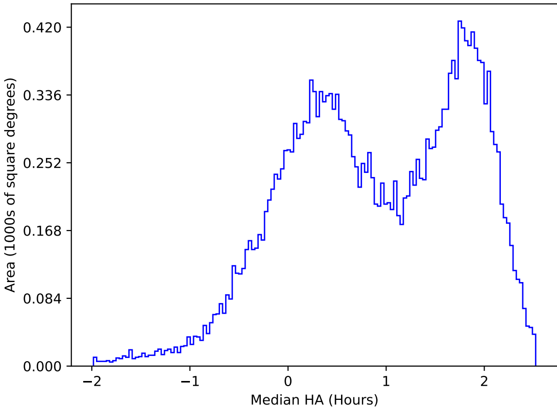
ddf_acor_sf25_lsf40_lsr10_v3.4_10yrs All sky u band: Median HA
