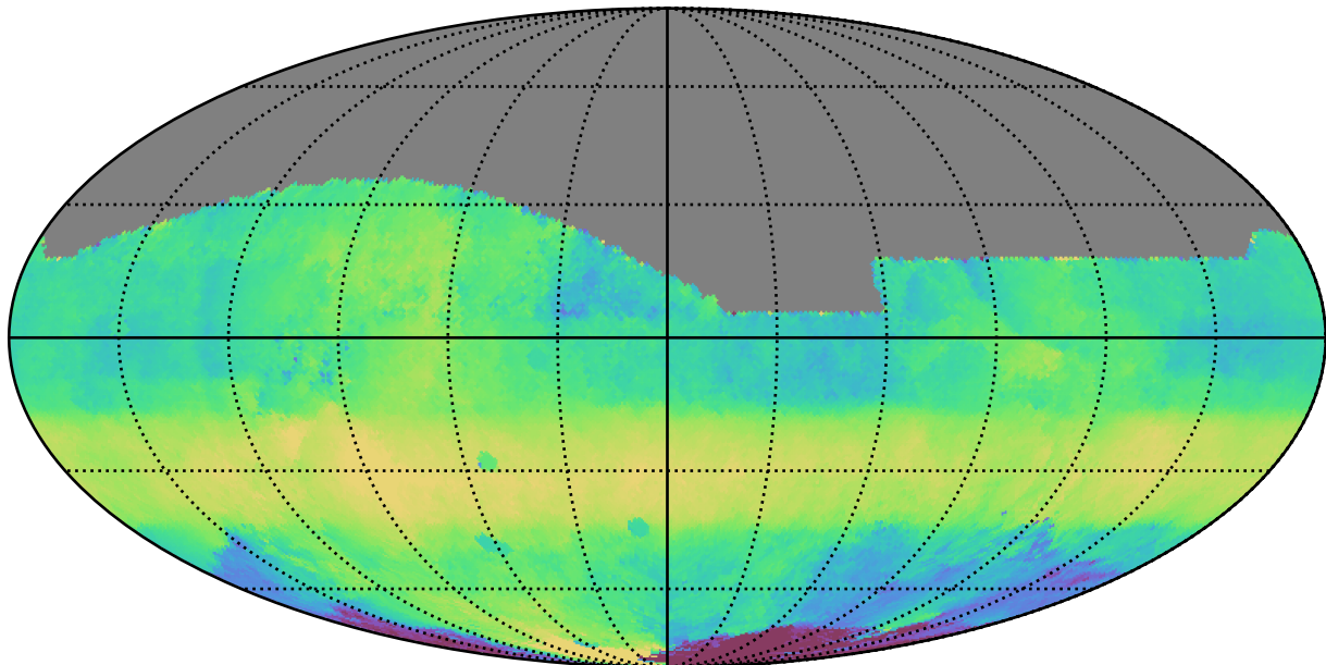
ddf_acor_sf25_lsf40_lsr10_v3.4_10yrs All sky r band: Median HA
