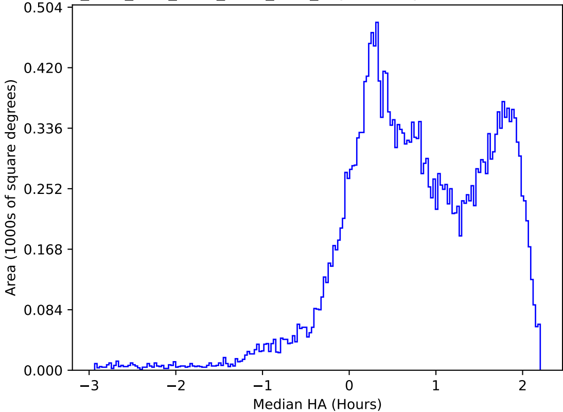
ddf_acor_sf25_lsf40_lsr10_v3.4_10yrs All sky r band: Median HA
