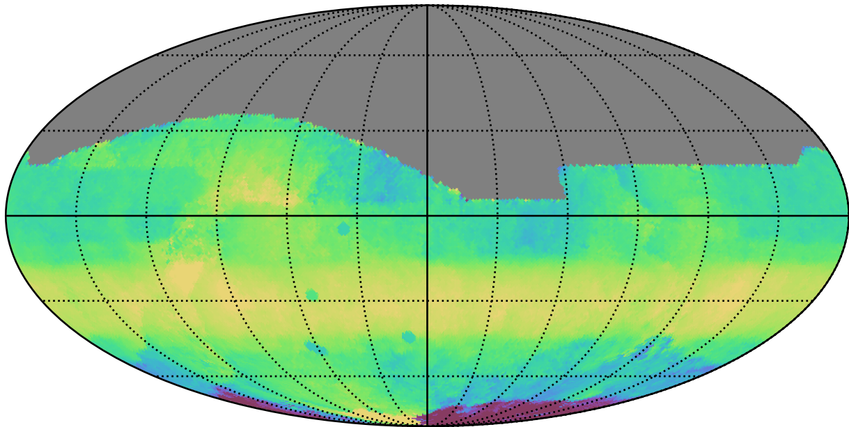
ddf_acor_sf25_lsf40_lsr10_v3.4_10yrs All sky i band: Median HA
