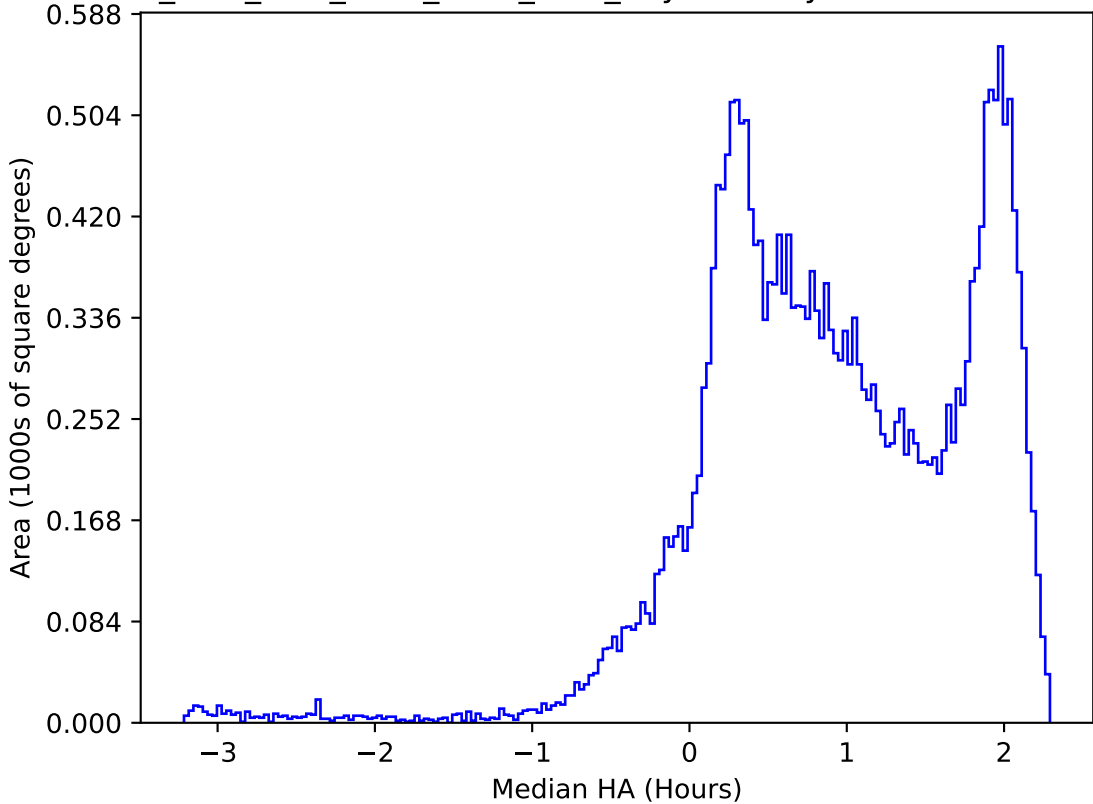
ddf_acor_sf25_lsf40_lsr10_v3.4_10yrs All sky i band: Median HA
