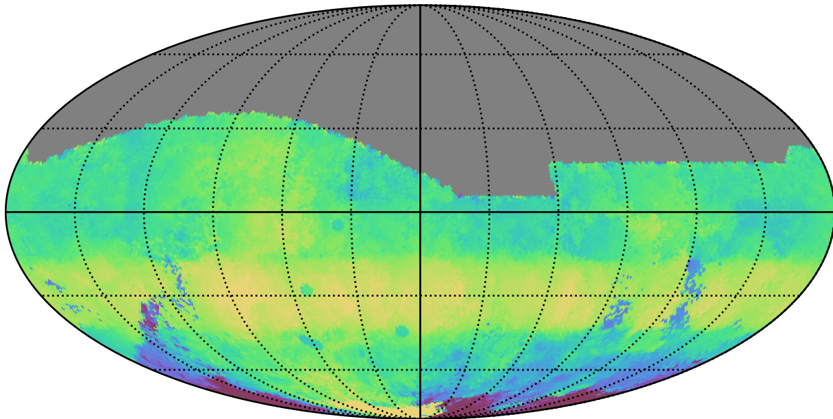
ddf_acor_sf25_lsf40_lsr10_v3.4_10yrs All sky g band: Median HA
