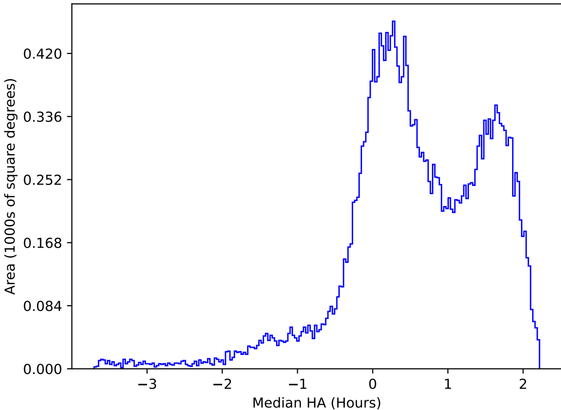
ddf_acor_sf25_lsf40_lsr10_v3.4_10yrs All sky g band: Median HA
