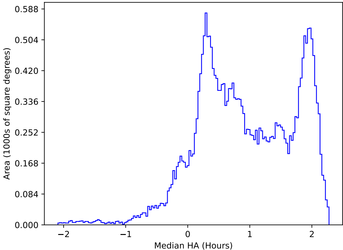
ddf_acor_sf25_lsf40_lsr10_v3.4_10yrs All sky all bands: Median HA
