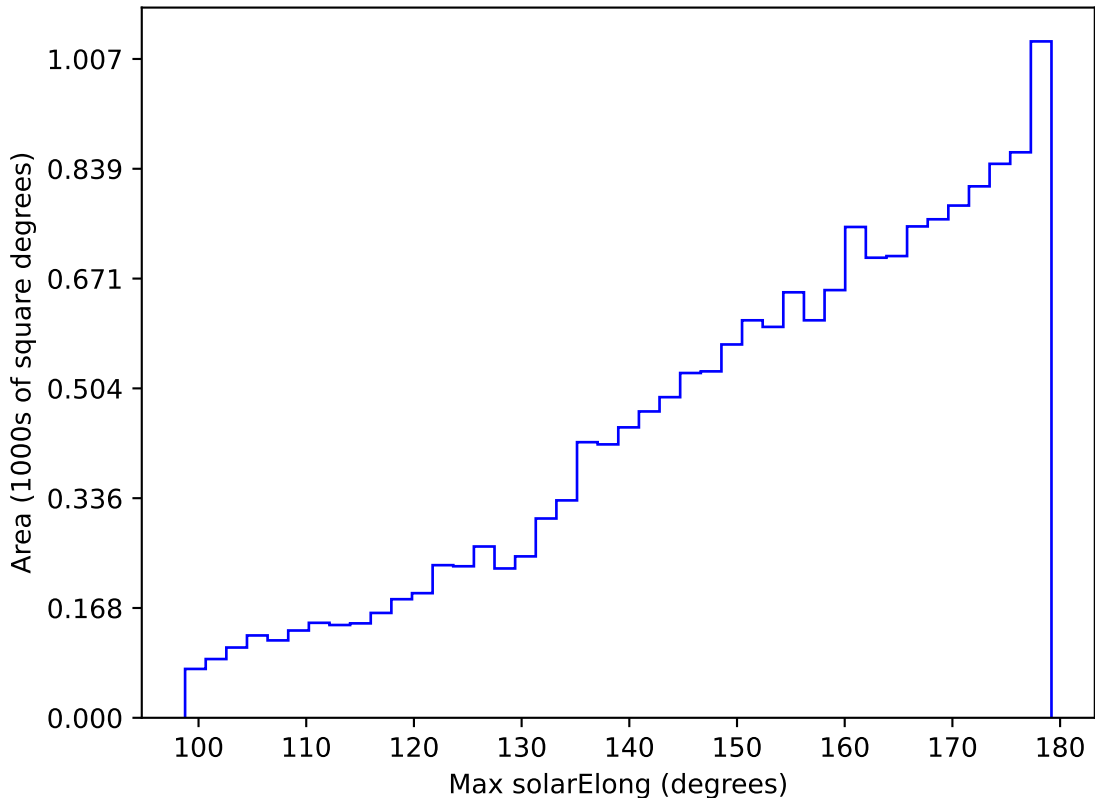
ddf_acor_sf25_lsf40_lsr10_v3.4_10yrs WFD y band: Max solarElong
