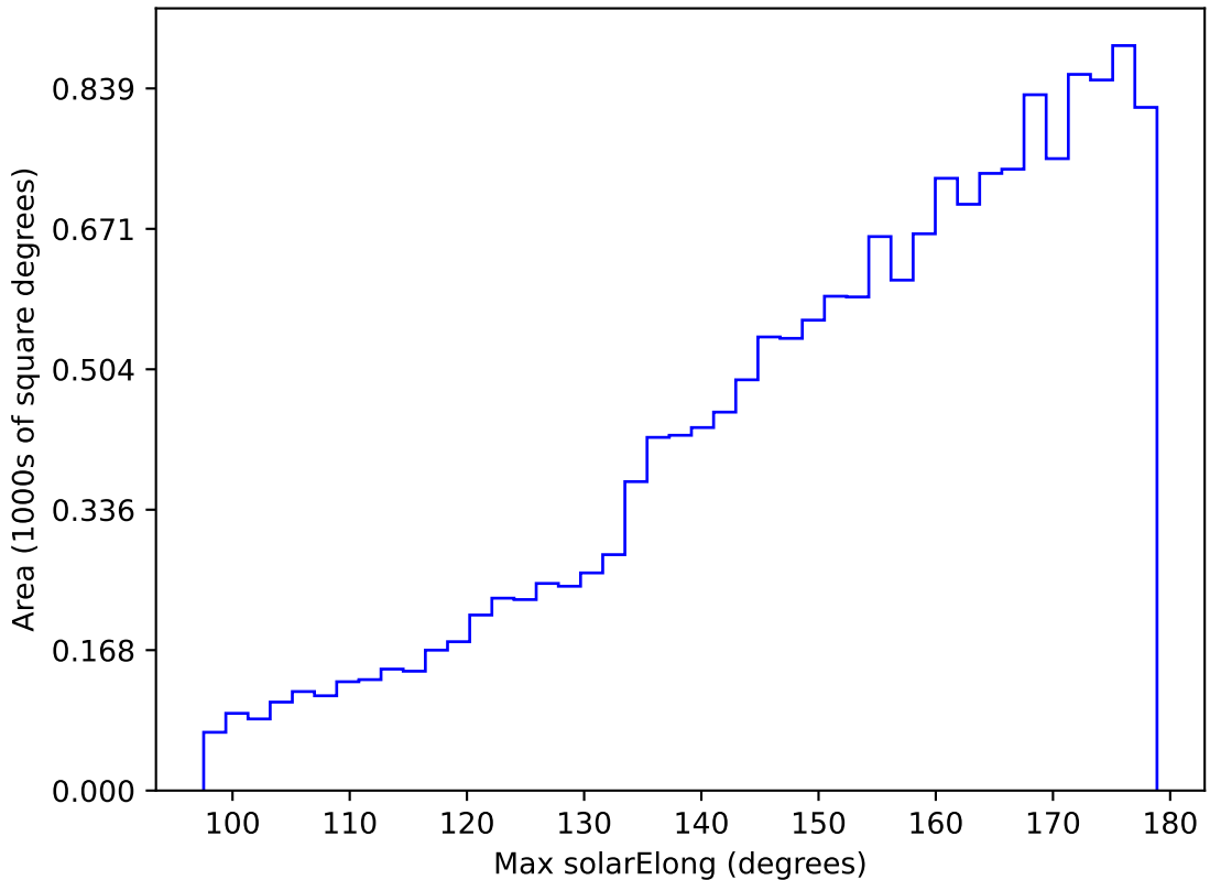
ddf_acor_sf25_lsf40_lsr10_v3.4_10yrs WFD u band: Max solarElong
