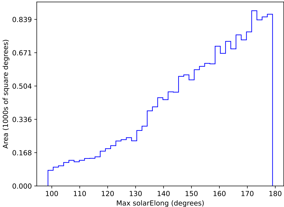
ddf_acor_sf25_lsf40_lsr10_v3.4_10yrs WFD g band: Max solarElong
