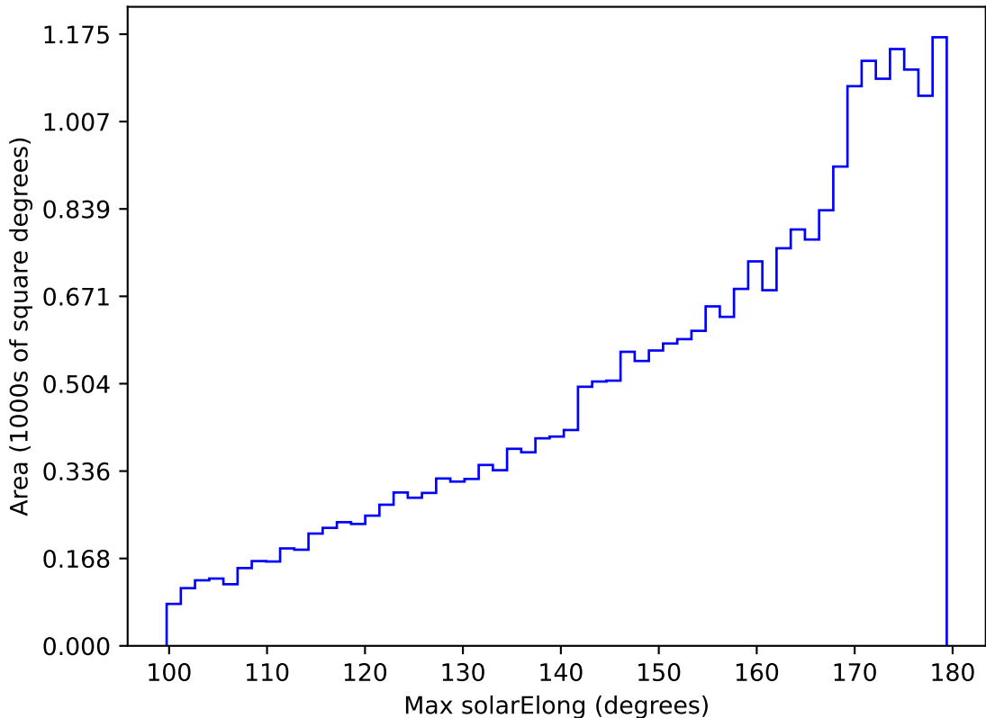
ddf_acor_sf25_lsf40_lsr10_v3.4_10yrs All sky z band: Max solarElong
