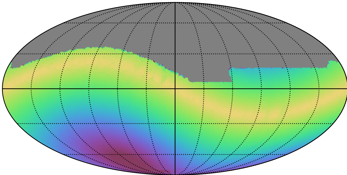
ddf_acor_sf25_lsf40_lsr10_v3.4_10yrs All sky r band: Max solarElong
