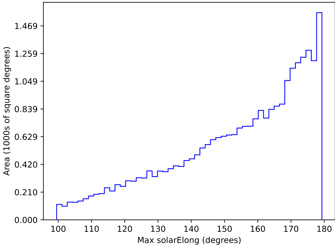
ddf_acor_sf25_lsf40_lsr10_v3.4_10yrs All sky r band: Max solarElong
