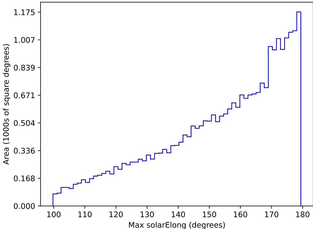
ddf_acor_sf25_lsf40_lsr10_v3.4_10yrs All sky i band: Max solarElong
