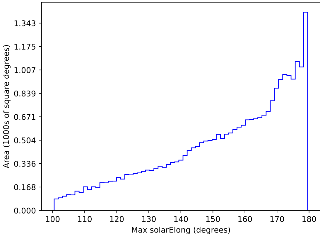
ddf_acor_sf25_lsf40_lsr10_v3.4_10yrs All sky all bands: Max solarElong
