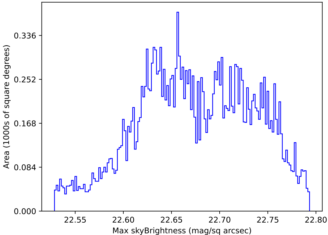
ddf_acor_sf25_lsf40_lsr10_v3.4_10yrs Yr 1 u band: Max skyBrightness
