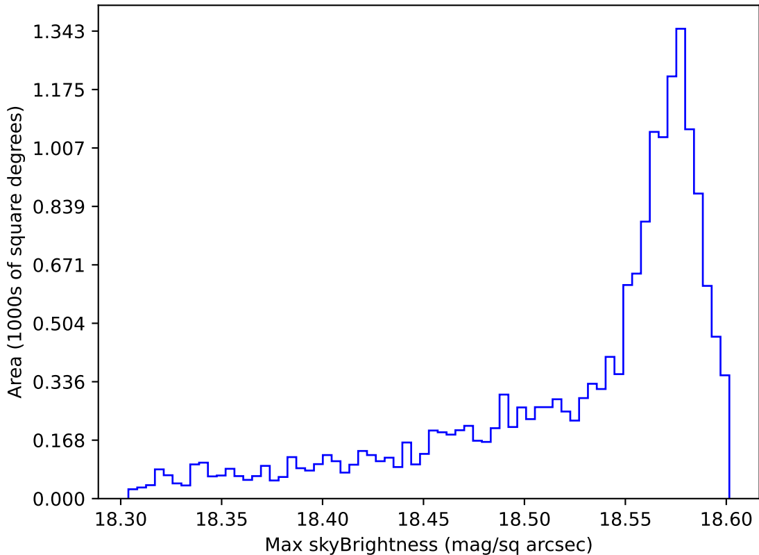
ddf_acor_sf25_lsf40_lsr10_v3.4_10yrs WFD y band: Max skyBrightness
