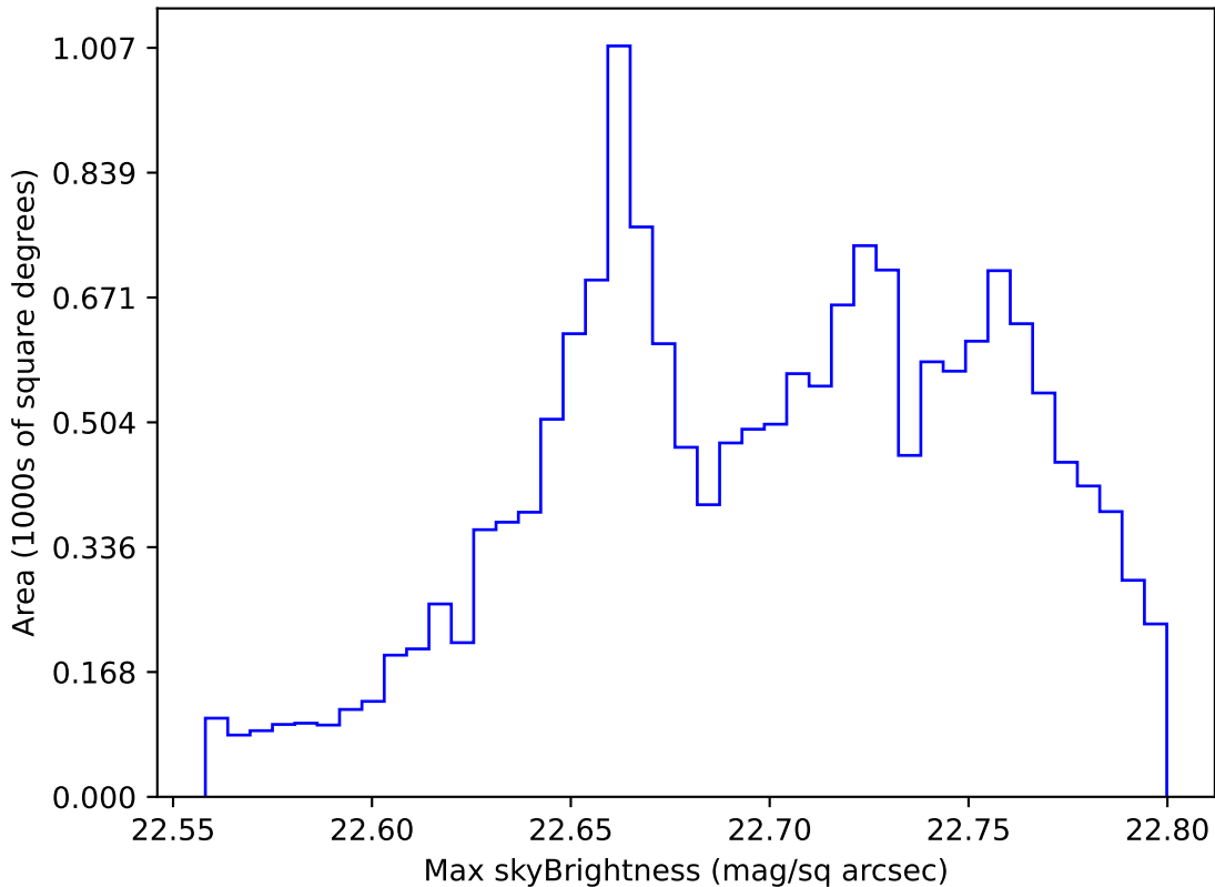
ddf_acor_sf25_lsf40_lsr10_v3.4_10yrs WFD u band: Max skyBrightness
