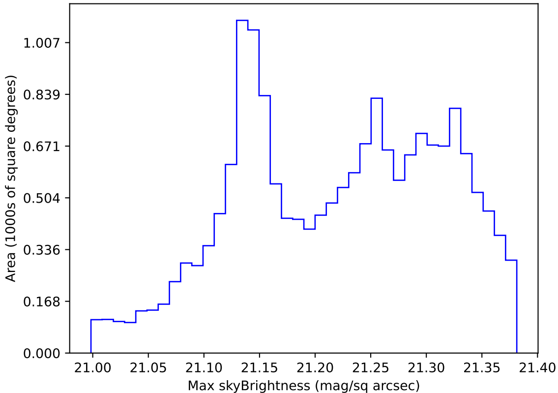
ddf_acor_sf25_lsf40_lsr10_v3.4_10yrs WFD r band: Max skyBrightness
